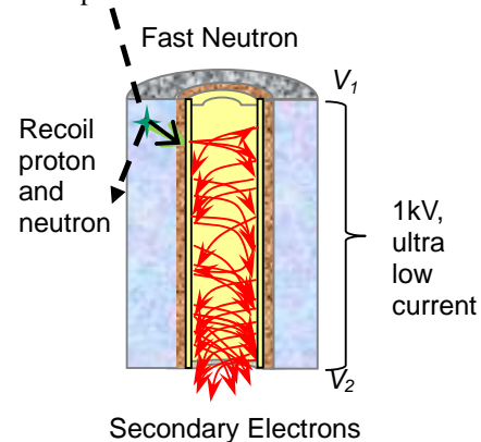
Fig. 7. Principle of fast neutron detection in hydrogen-rich plastic MCP. The recoil proton releases secondary electrons upon collision with the pore walls, which are coated with conduction and emission ALD films. The rest of detection process is similar to photon detection.
