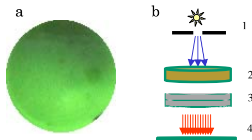
Fig. 4. (a) Photograph of the phosphor screen with detector under UV illumination. No noise spots or artifacts from PMMA MCP are observed. The defects on the image are due to the phosphor internal features. (b) Schematic diagram of the pulse counting detector configuration (not to scale). 1 – UV light source with an aperture, 2 – PMMA MCP, 3 – standard lead glass MCP (or a chevron stack) used for post-amplification of electron signal produced by the PMMA MCP. 4 – phosphor screen/charge collecting anode.
