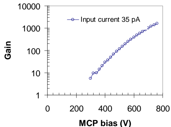
Fig. 3. PMMA MCP gain as a function of applied bias measured in a current amplification mode under full-field electron illumination. 35 pA input current was spread over the entire MCP active area of \sim 20 \text{ mm} containing \sim 7.4 \times 10^4 pores ( \sim 3000 input electrons/pore/s).
