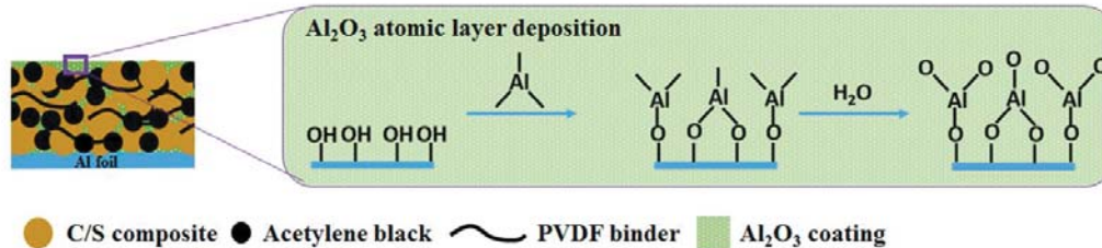
Fig. S1. Schematic of atomic layer deposition Al 2 O 3 coating on carbon-sulfur cathode. A typical Al 2 O 3 ALD chemical reaction is conducted using H 2 O and TMA as precursors.
